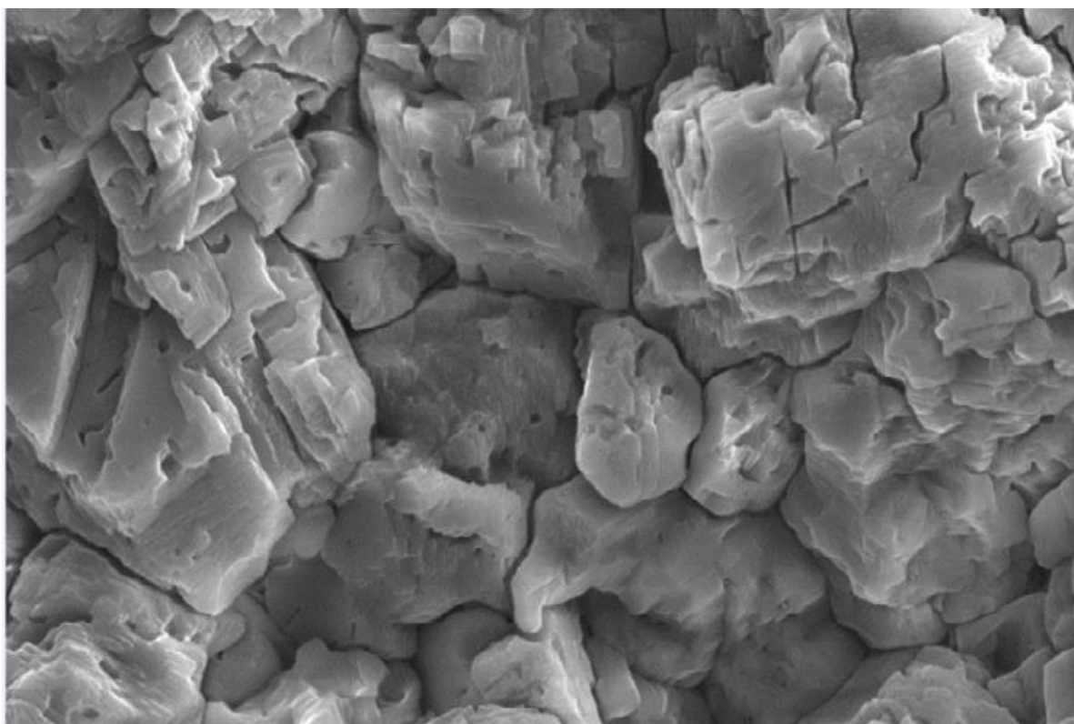
Scanning Electron Microscope (SEM) image of Lanthanum nanoparticles with 50000x zoom.
