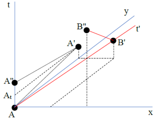
Figure 2. Lorentz transformation for photon reflection experiments
