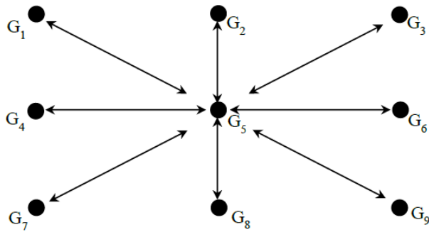
Figure 9. Homogeneous universe in an unlimited space
