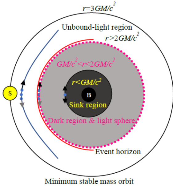
Figure 5. Regions of a black hole
