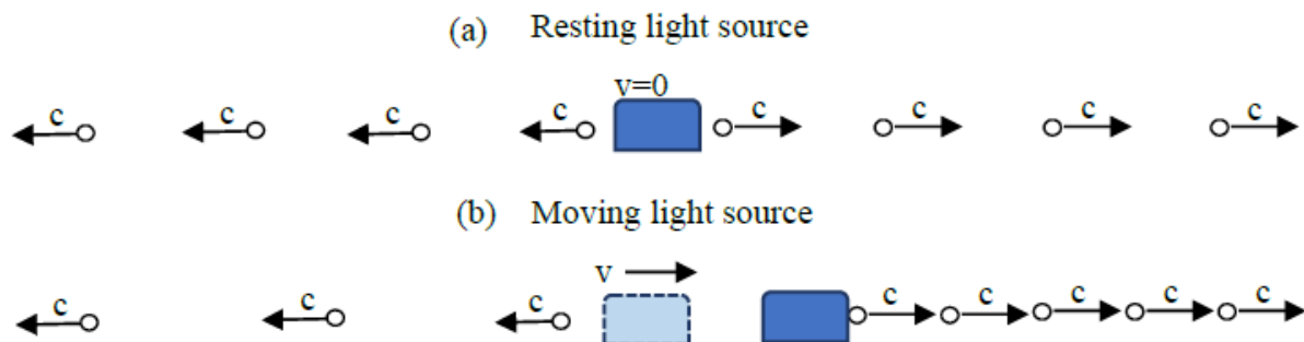
Figure 1. Speed of light source, photon density, and relative mass
