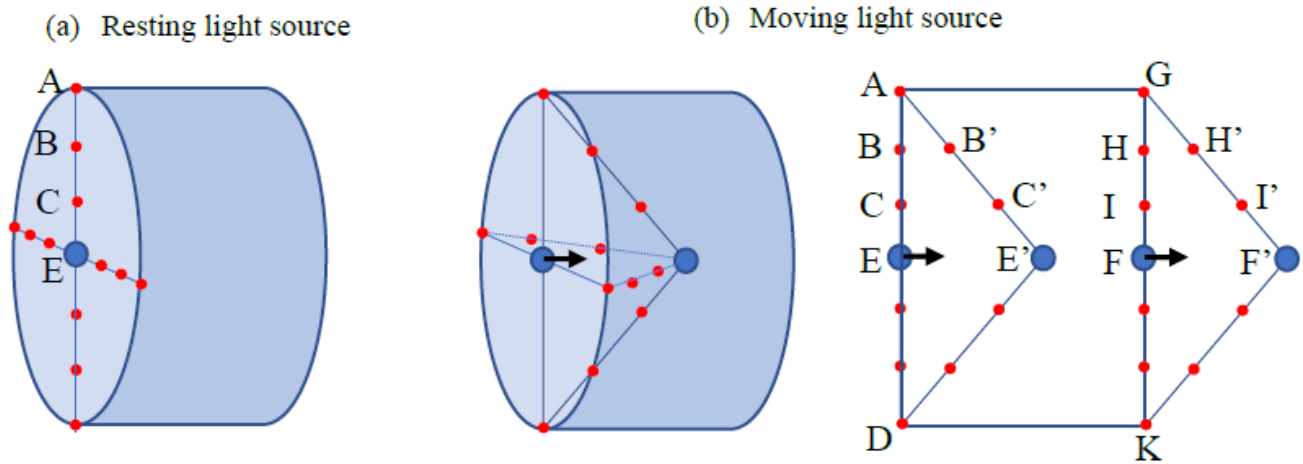
Figure A2. Photon density at the cross section
