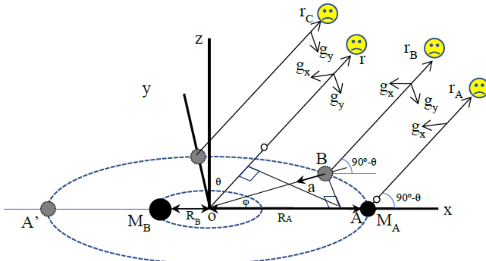
Figure 7. Gravity field change caused by binary stars
