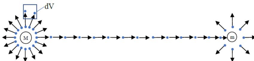
Figure 3. Photon density and gravitational force
