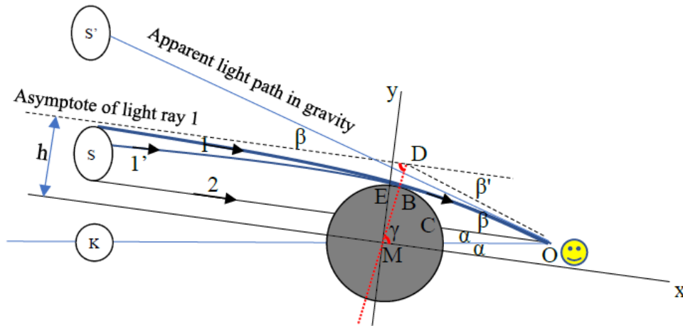
Figure 4. Calculating deflection angle in a gravity field
