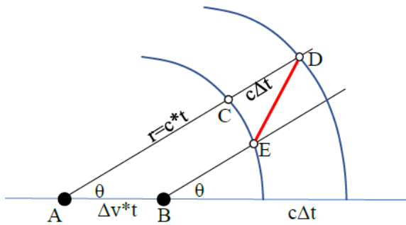
Figure 6. Gravity field change caused by motion of mass
