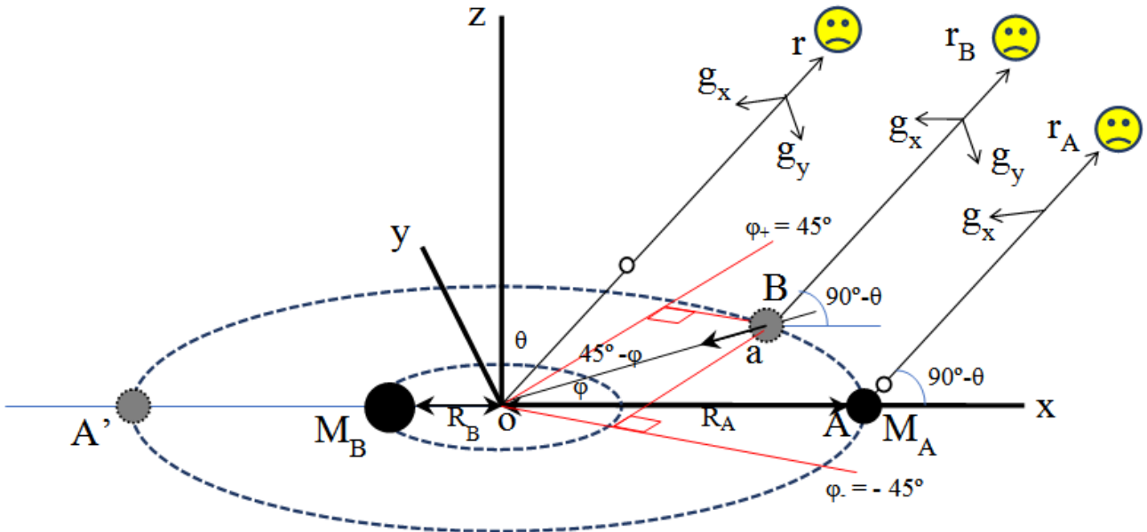
Figure 8. Gravity field change caused by binary stars
