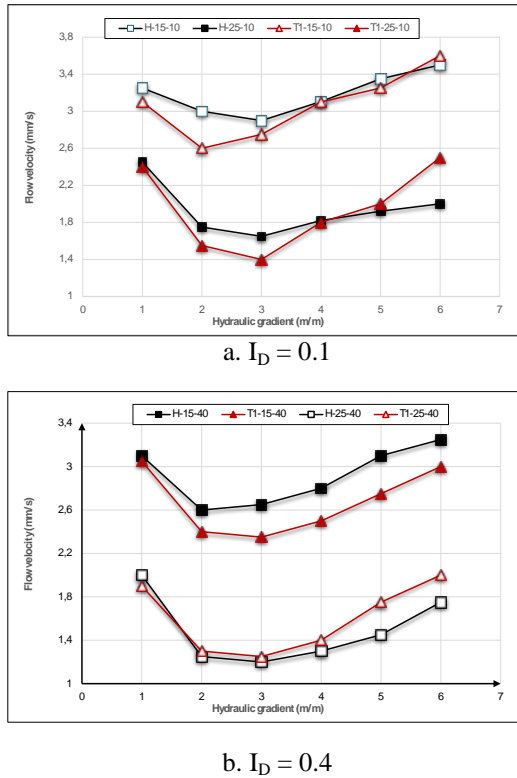
Figure 4. Flow velocity versus hydraulic gradient
