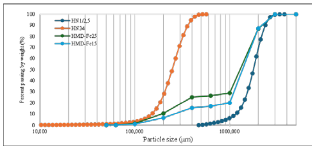
Figure 1. Particles size distribution curves of basic material and reconstituted samples
