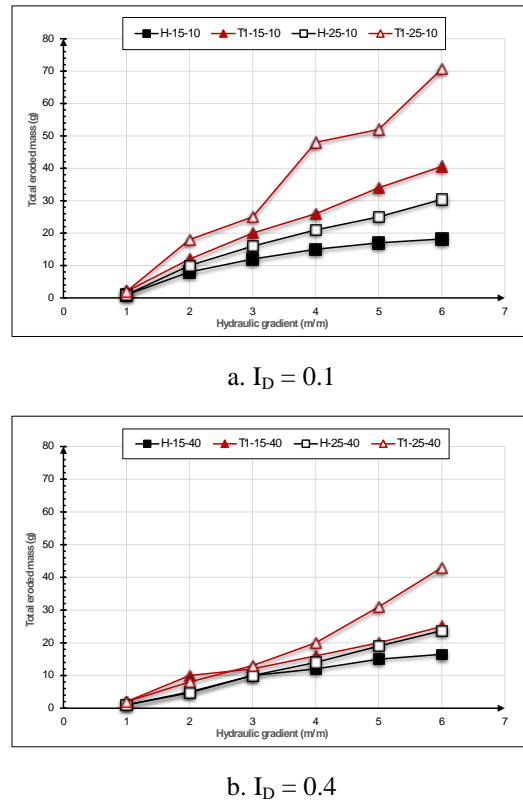
Figure 5. Total eroded mass versus hydraulic gradient – Type 1 Heterogeneity
