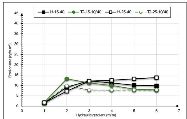
Figure 8. Erosion rate versus hydraulic gradient – Type 2 Heterogeneity
