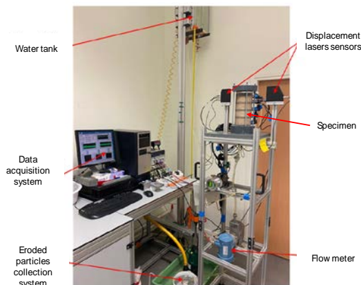
Figure 2. Suffusion column experimental apparatus
