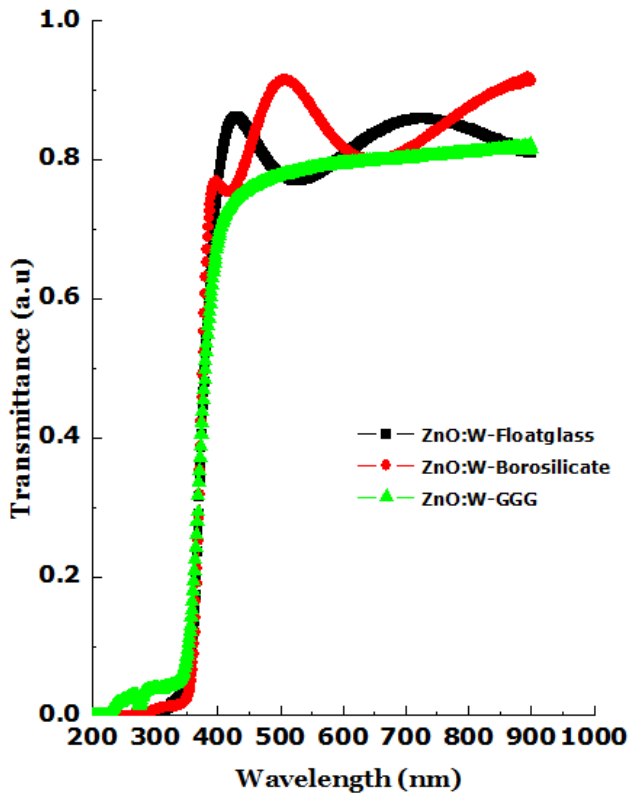
Figure 4. Transmission spectrums for the ZnO:W thin film grown on different glass substrates
