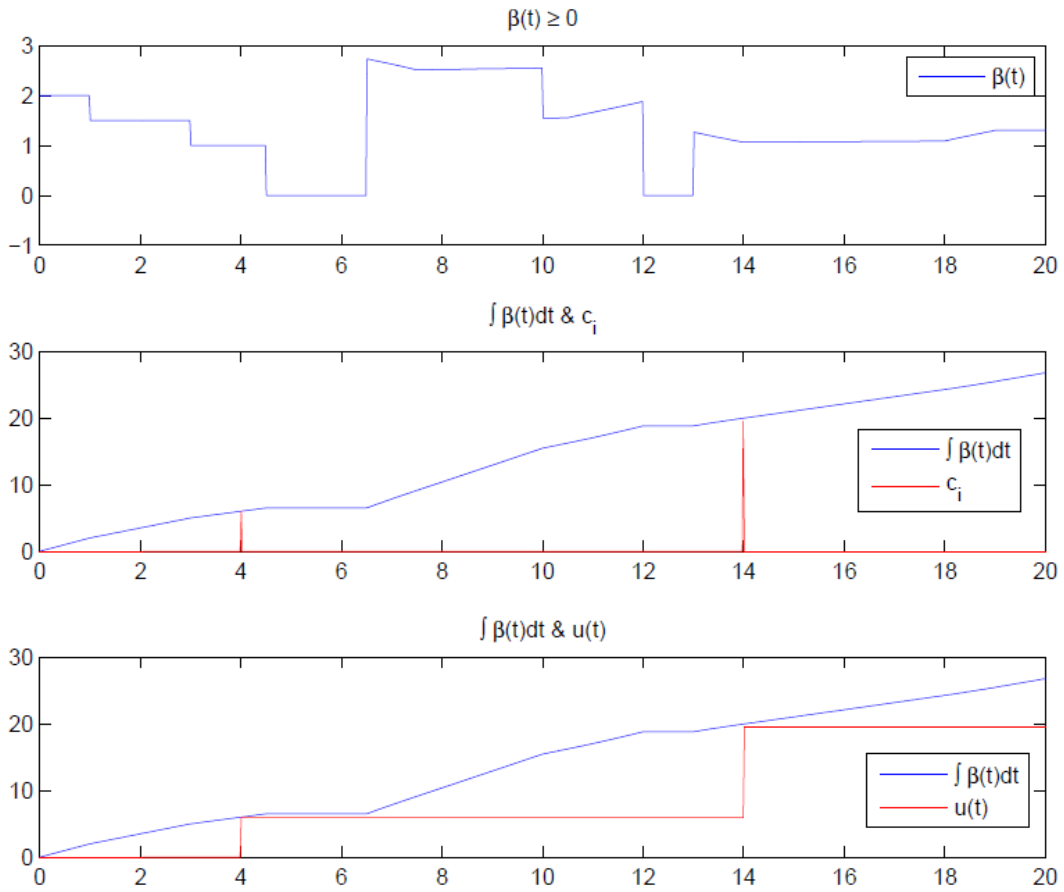
Figure 5. Checking if the constraints are verified for Example 1
