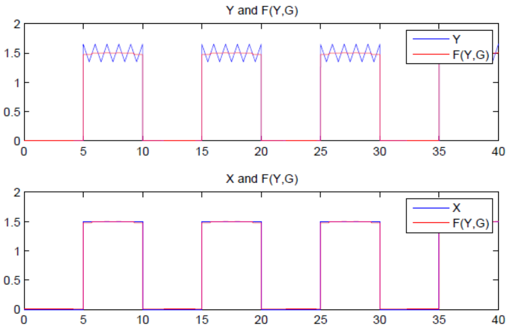
Figure 2. Filtering by using TVD
