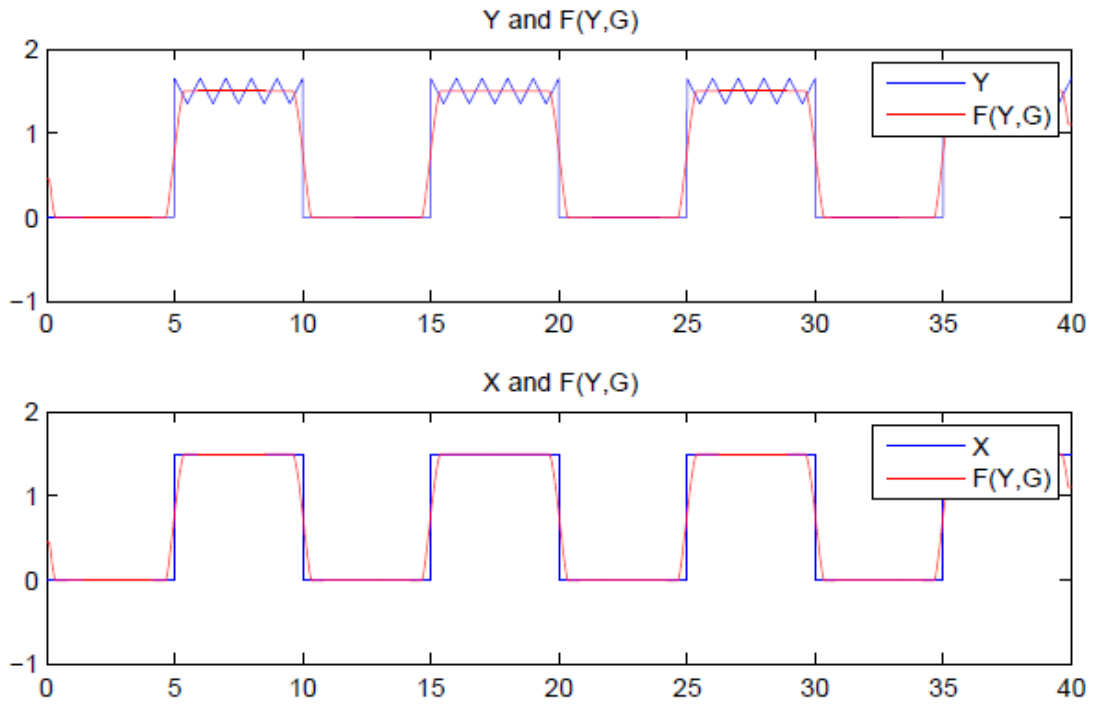
Figure 3. Filtering by using thresholding method
