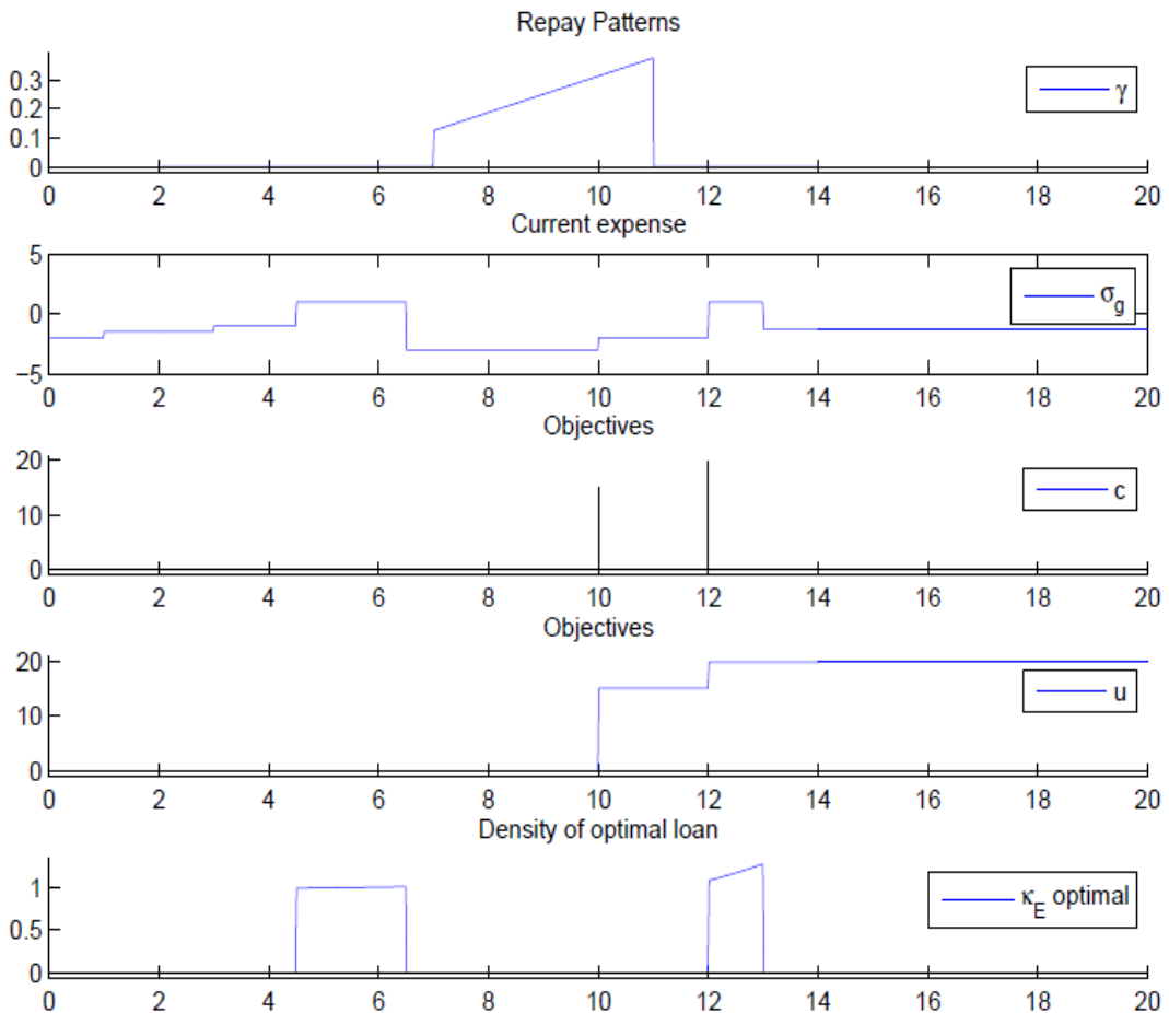
Figure 6. Optimal loan \kappa_E obtained for given: repayment pattern \gamma , objectives c and current spending \sigma_g
