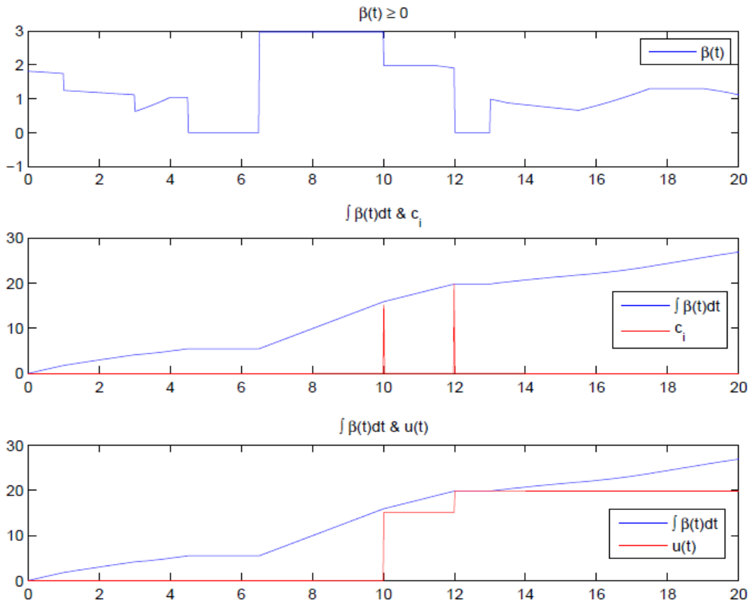
Figure 7. Checking if the constraints are verified for Example 2
