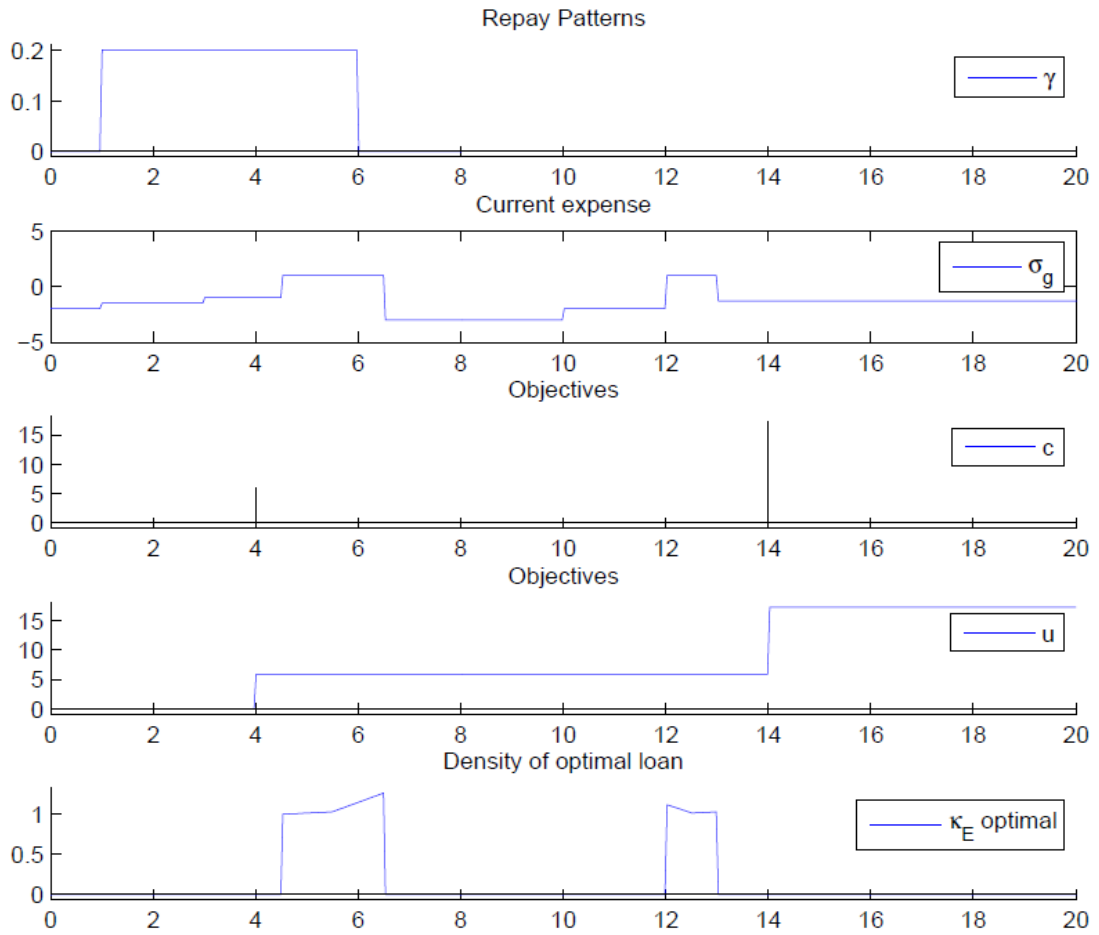
Figure 4. Example 1. Optimal loan \kappa_E obtained for given: repayment pattern \gamma , objectives c and current spending \sigma_g
