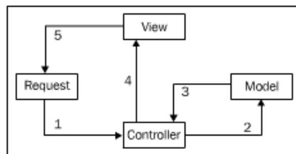
Figure 3. MVC architecture [12]
